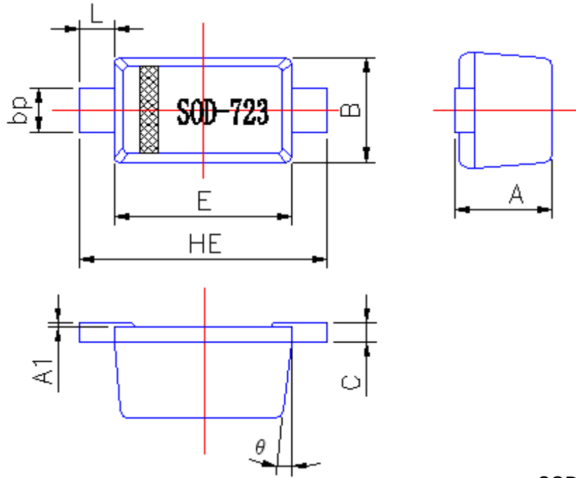
SOD-723 1.0
