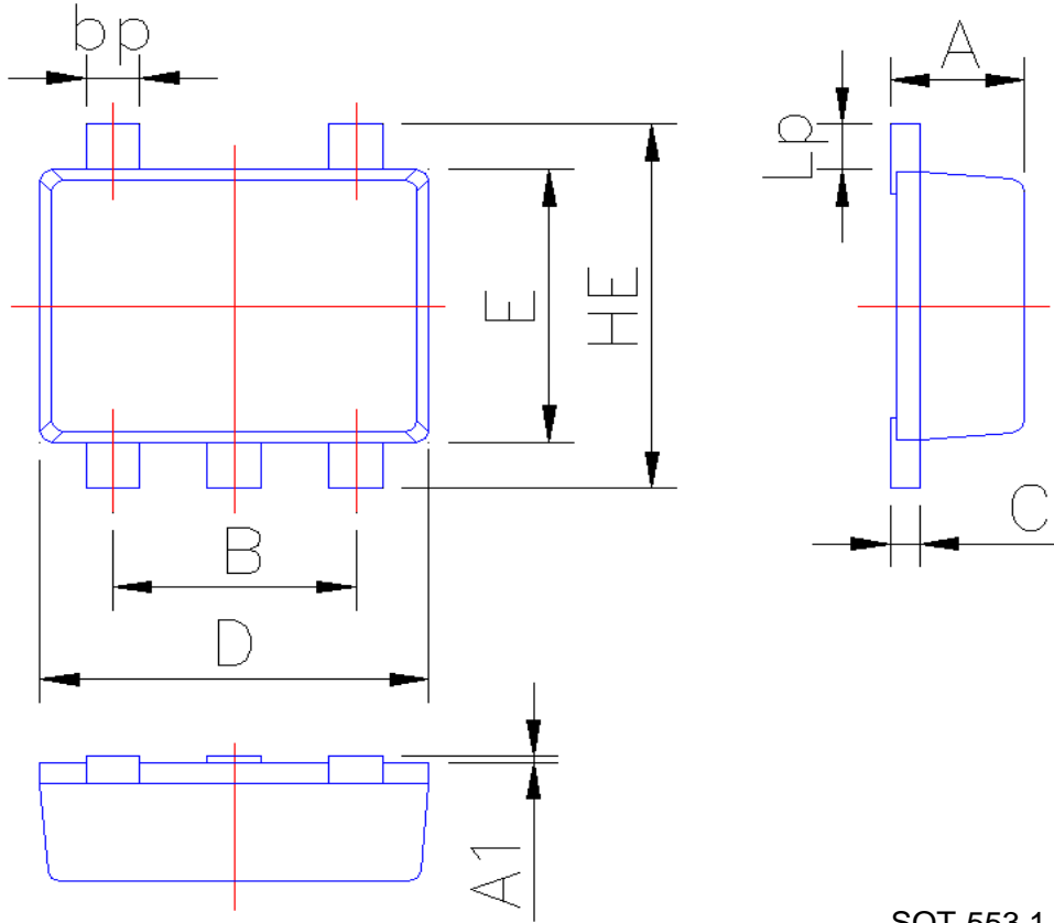
SOT-553 1.0
