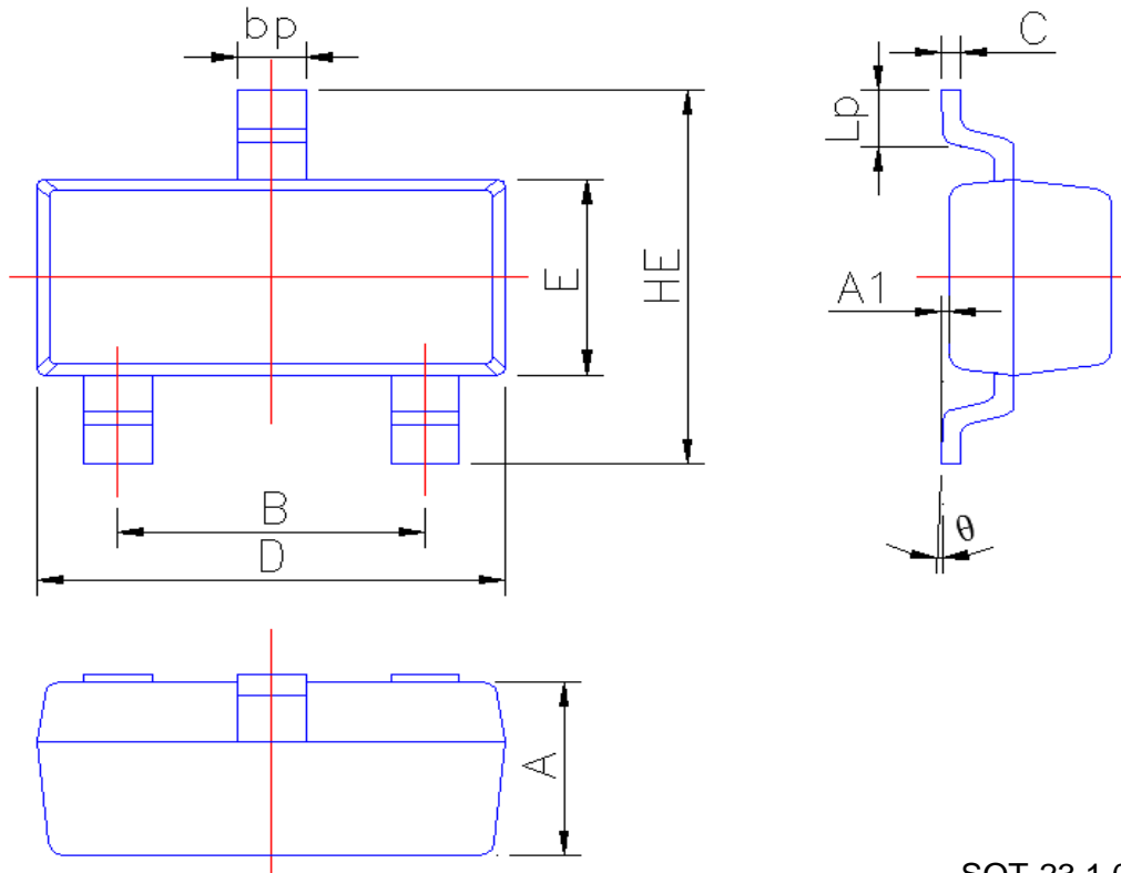
SOT-23 1.0
