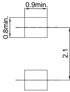
SOD-323
