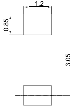
SOD-123
