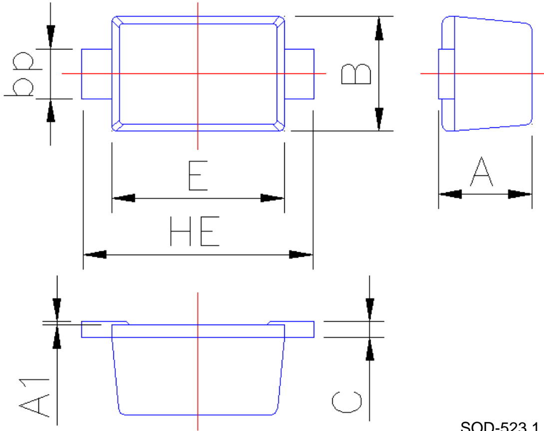
SOD-523 1.0
