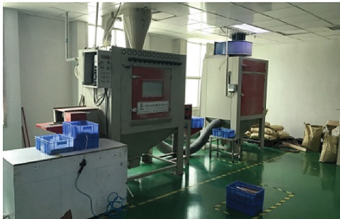
Punching burr sandblasting machine
