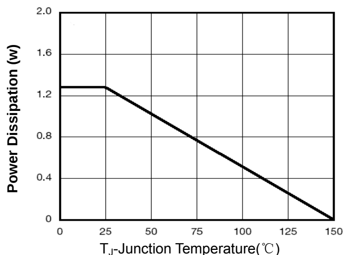
Figure 6 Power De-ratin
